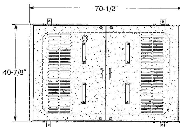
Plan Transformer Frame and Cover Assembly
